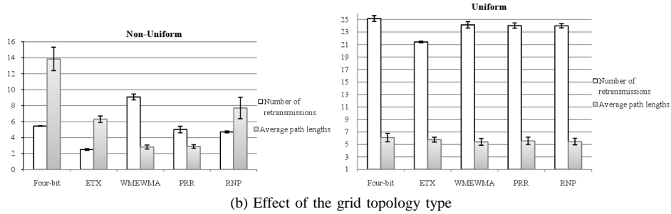
Fig. 13. Performance comparison in terms of number of retransmissions and average path length
