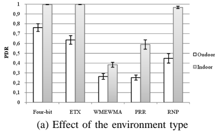
Fig. 11. Performance comparison in terms of Packet Delivery Rate (PDR)
